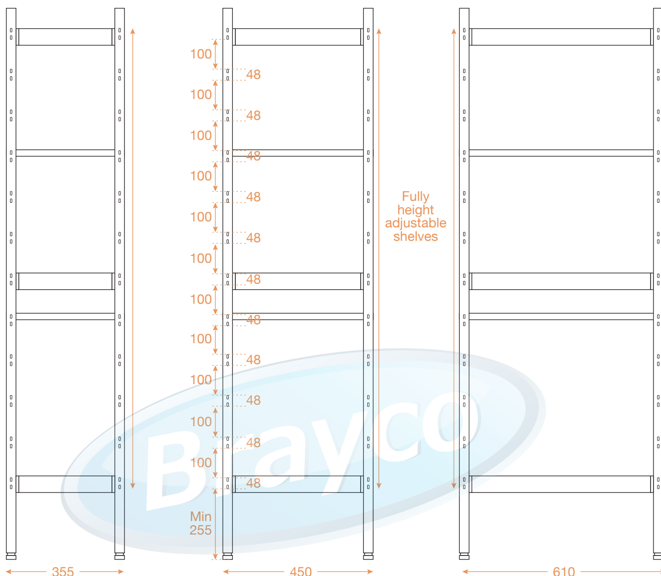
355mm Deep
