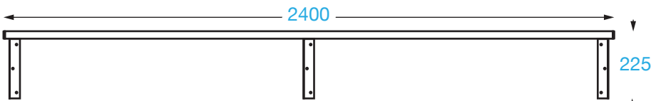
FRONT
