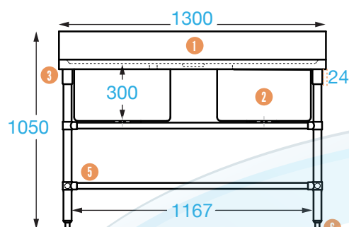
FRONT
