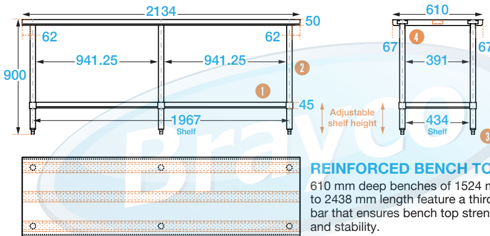
FRONT
